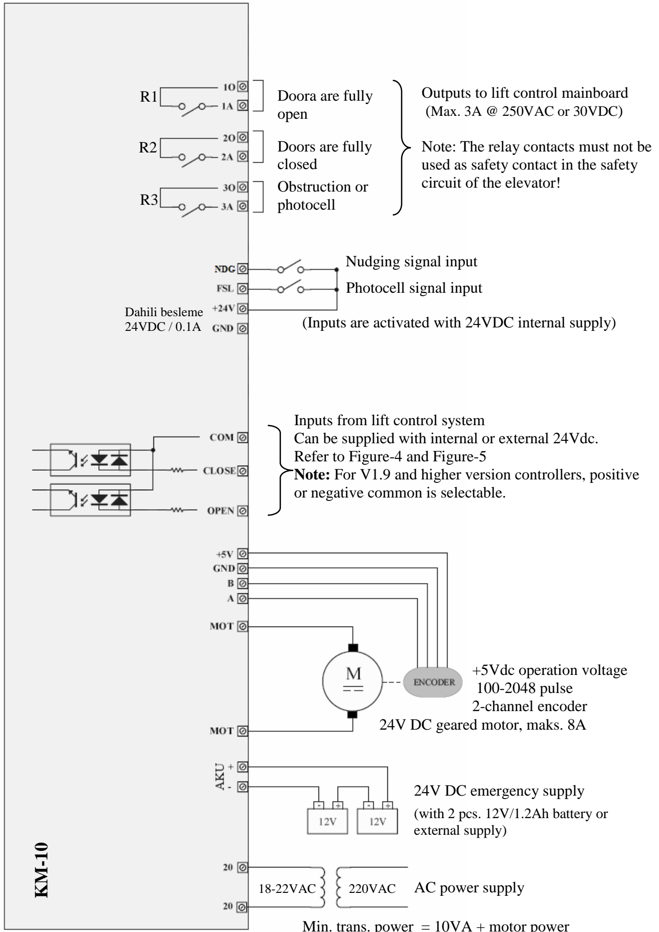
Figure-3: Connection diagram
