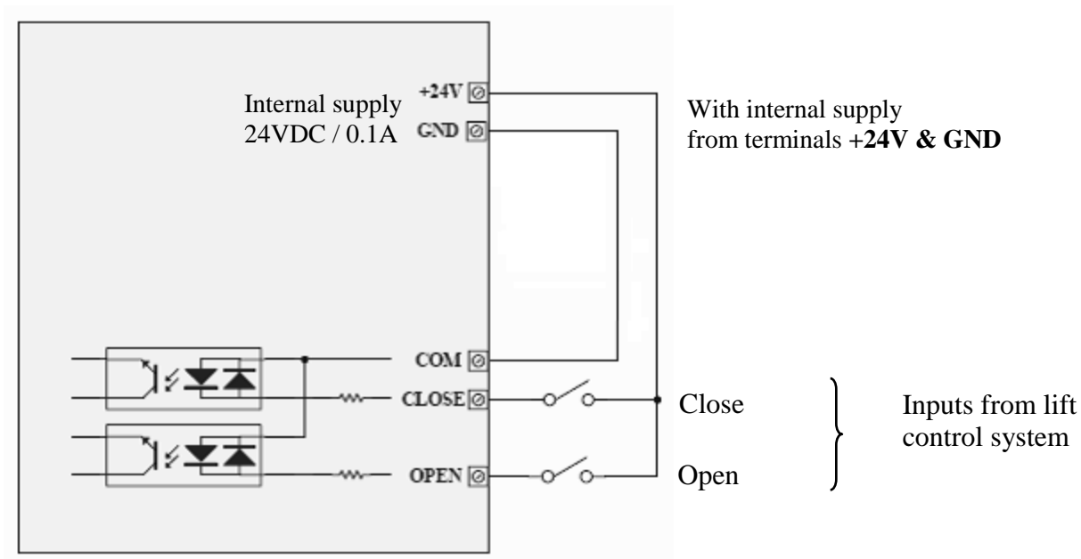
Figure-4: Control inputs connection with internal supply
