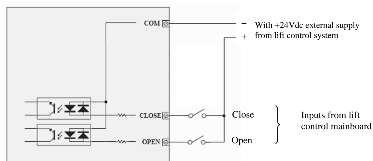
Figure-5: Control inputs connection with external supply
