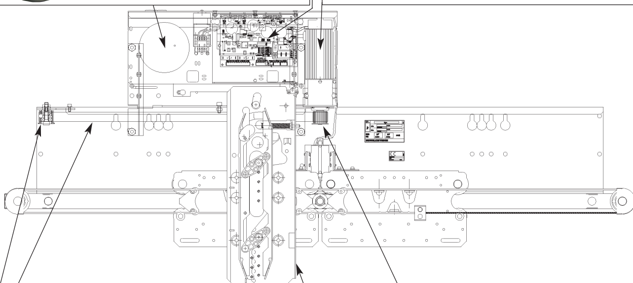
3215.05.7400 Belt for ECO door Cinghia per porta ECO 3201.05.7315 Belt for MIDI/SUPRA door Cinghia per porta MIDI/SUPRA
